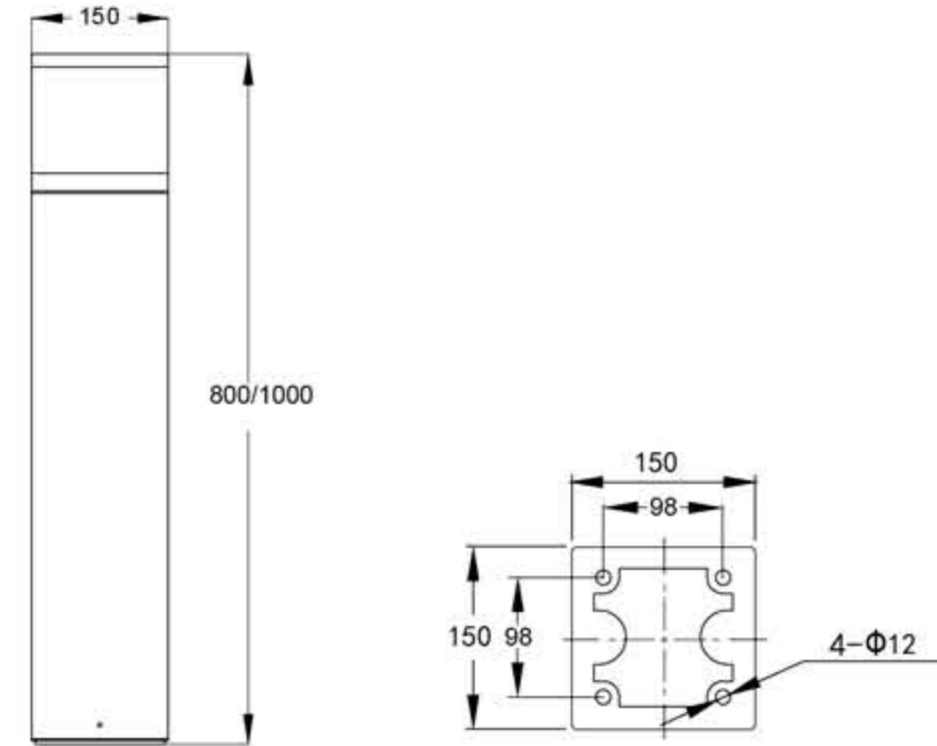
灯具尺寸 Product Dimensions(mm)
