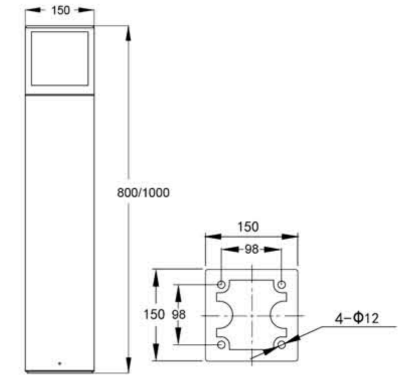
灯具尺寸 Product Dimensions(mm)
